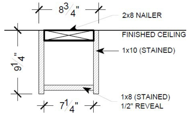
1/2" Reveal Beam Detail
