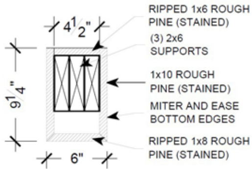
Mitered Corner Beam Detail
